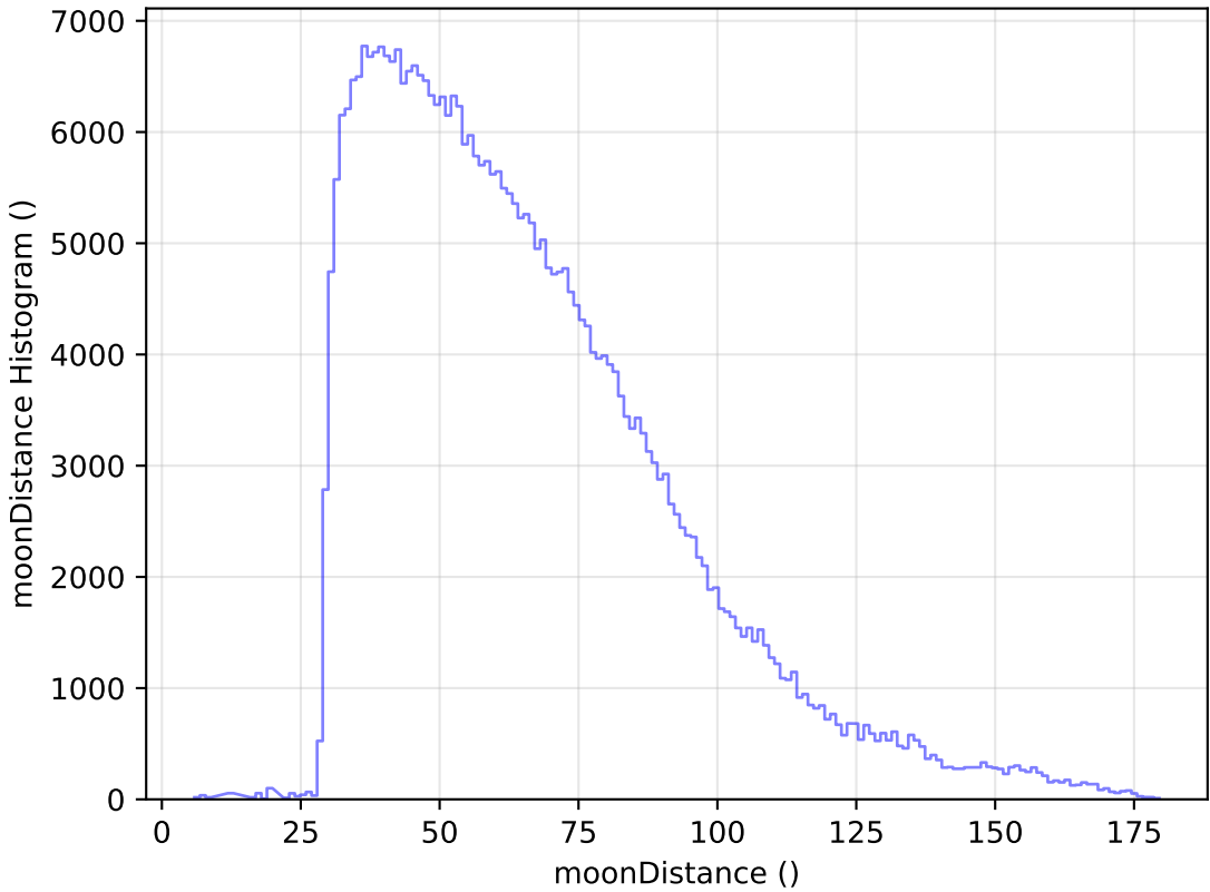
too_elab_r64_d3_griz_v3.4_10yrs All sky y band: moonDistance Histogram
