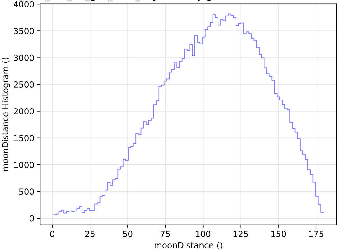
too_elab_r64_d3_griz_v3.4_10yrs All sky g band: moonDistance Histogram
