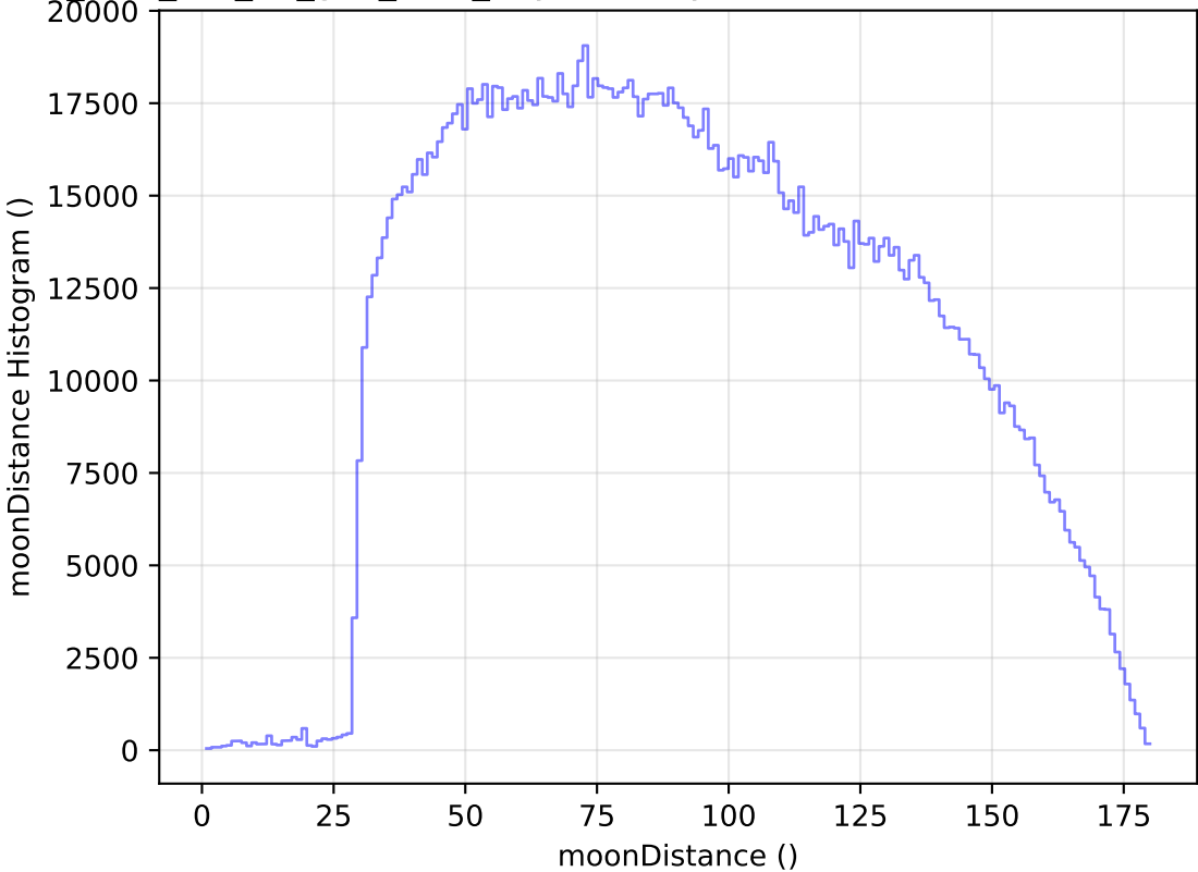
too_elab_r64_d3_griz_v3.4_10yrs All sky all bands: moonDistance Histogram
