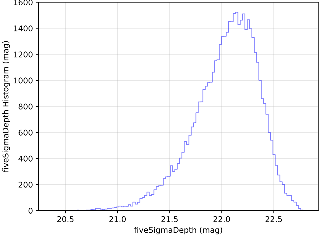
too_elab_r64_d3_griz_v3.4_10yrs Yr 1 y band: fiveSigmaDepth Histogram
