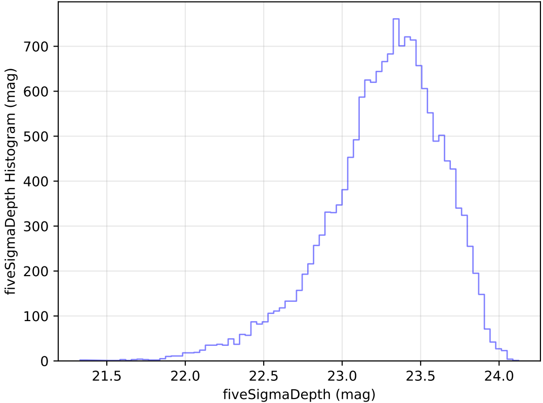
too_elab_r64_d3_griz_v3.4_10yrs Yr 1 u band: fiveSigmaDepth Histogram
