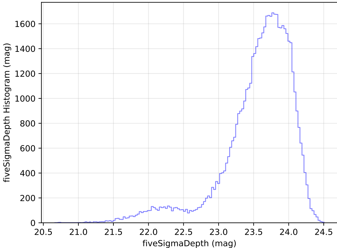
too_elab_r64_d3_griz_v3.4_10yrs Yr 1 i band: fiveSigmaDepth Histogram
