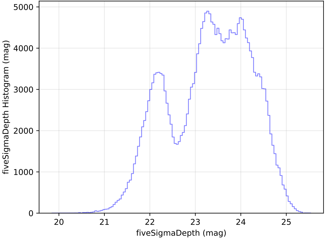
too_elab_r64_d3_griz_v3.4_10yrs Yr 1 all bands: fiveSigmaDepth Histogram
