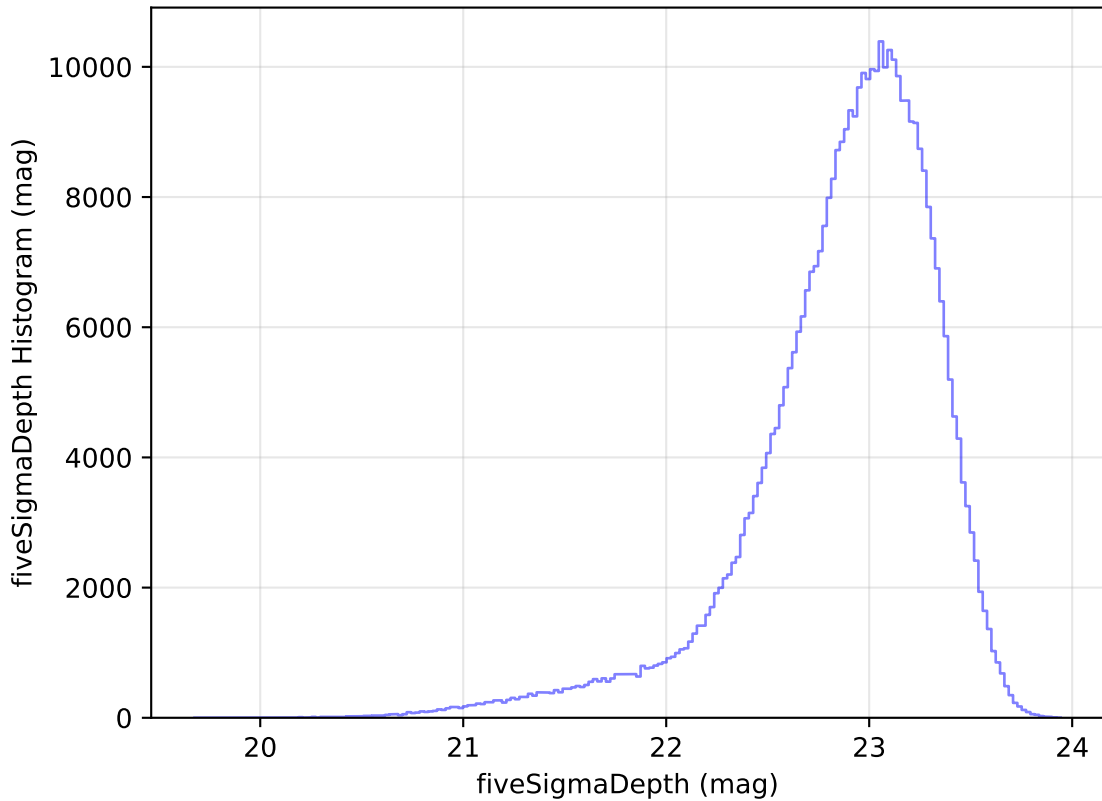
too_elab_r64_d3_griz_v3.4_10yrs WFD z band: fiveSigmaDepth Histogram
