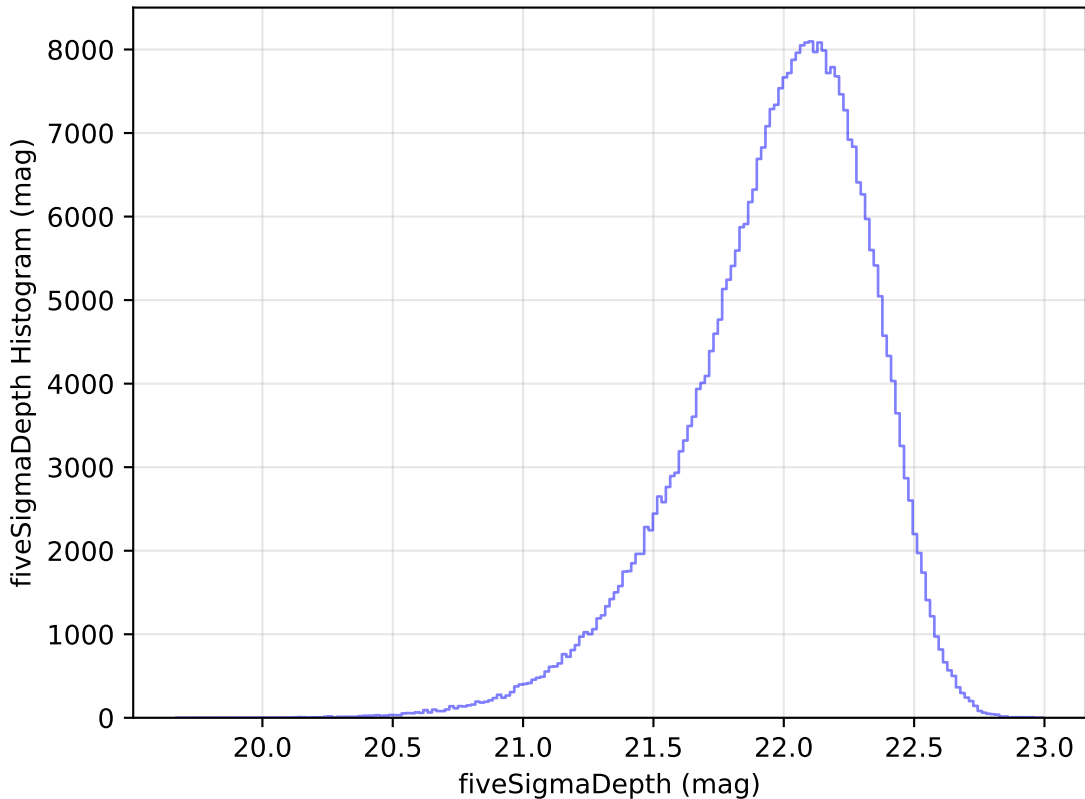
too_elab_r64_d3_griz_v3.4_10yrs WFD y band: fiveSigmaDepth Histogram
