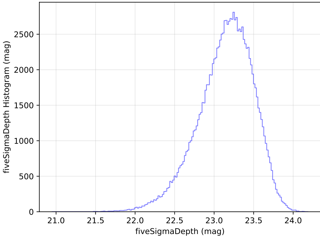
too_elab_r64_d3_griz_v3.4_10yrs WFD u band: fiveSigmaDepth Histogram
