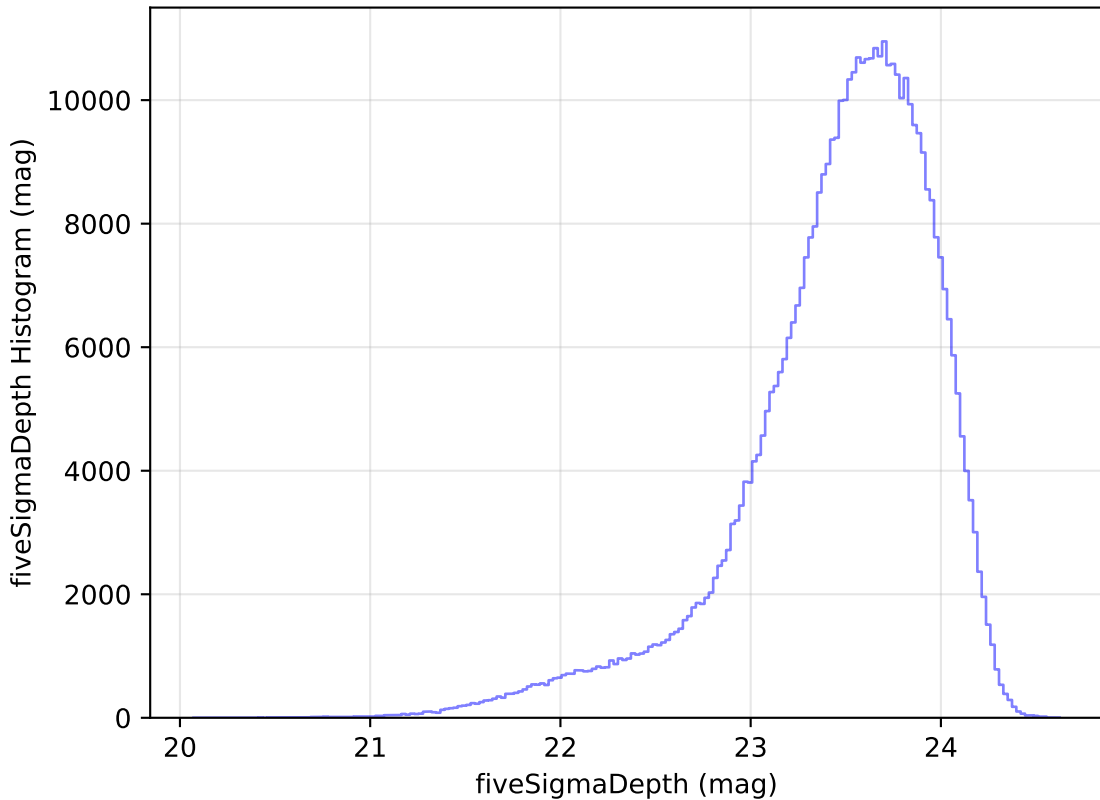
too_elab_r64_d3_griz_v3.4_10yrs WFD i band: fiveSigmaDepth Histogram
