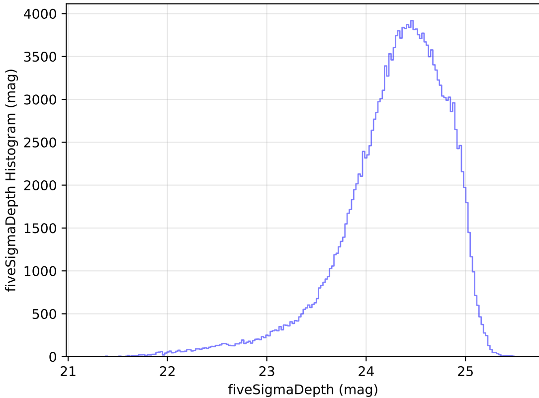
too_elab_r64_d3_griz_v3.4_10yrs WFD g band: fiveSigmaDepth Histogram
