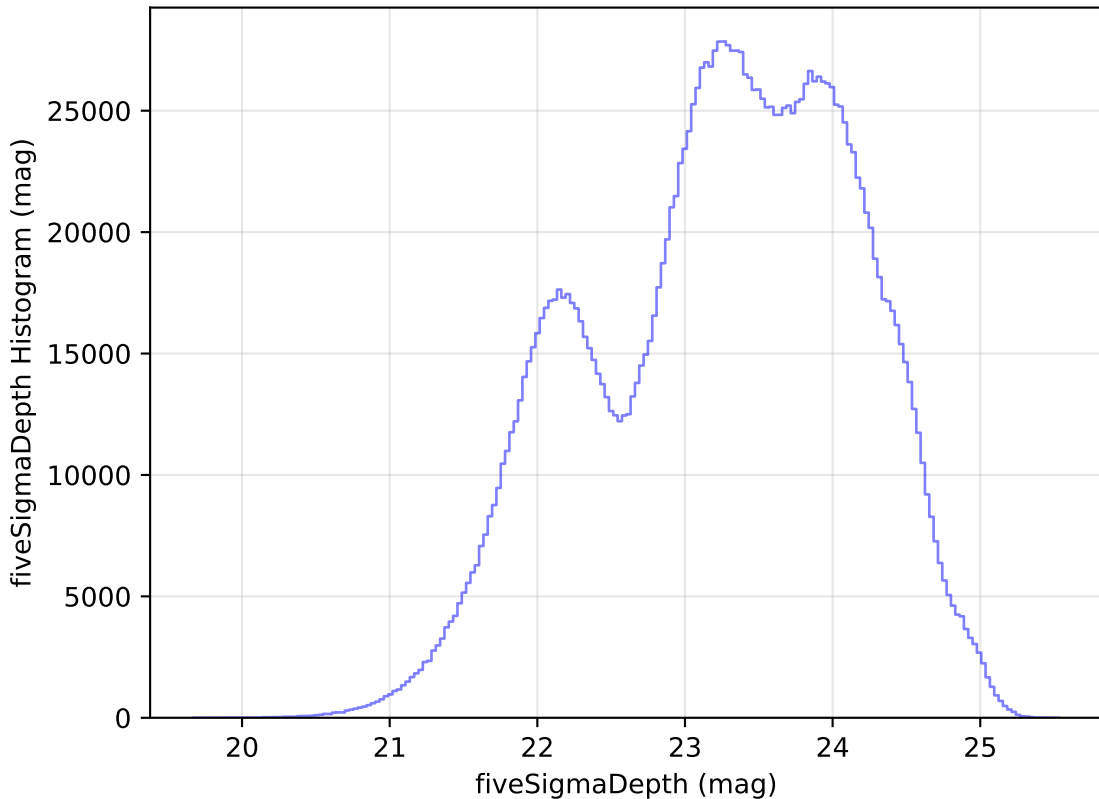
too_elab_r64_d3_griz_v3.4_10yrs WFD all bands: fiveSigmaDepth Histogram
