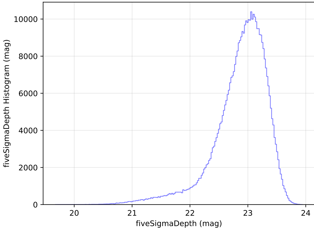
too_elab_r64_d3_griz_v3.4_10yrs All sky z band: fiveSigmaDepth Histogram
