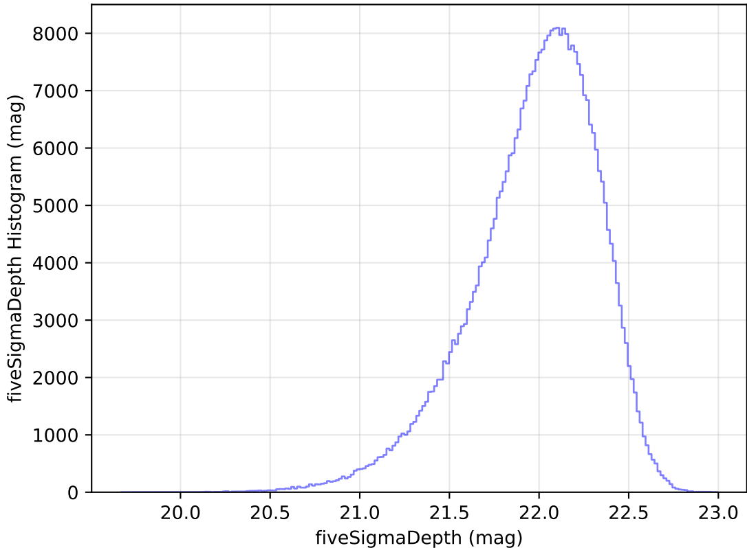
too_elab_r64_d3_griz_v3.4_10yrs All sky y band: fiveSigmaDepth Histogram
