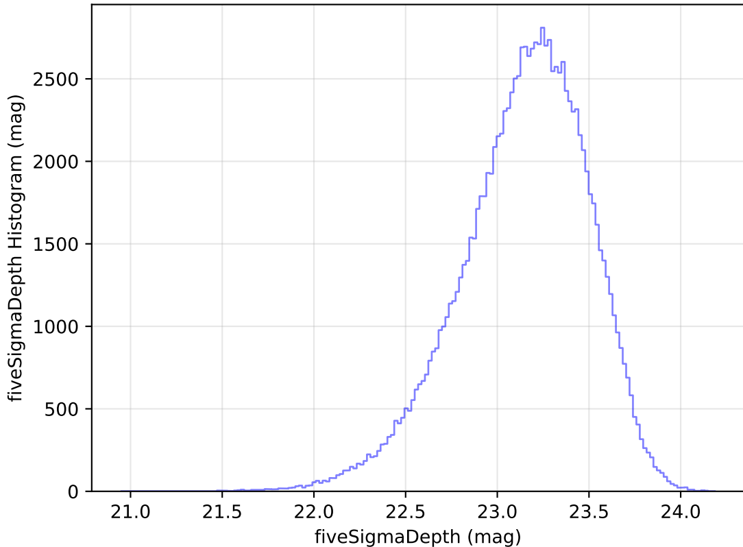
too_elab_r64_d3_griz_v3.4_10yrs All sky u band: fiveSigmaDepth Histogram
