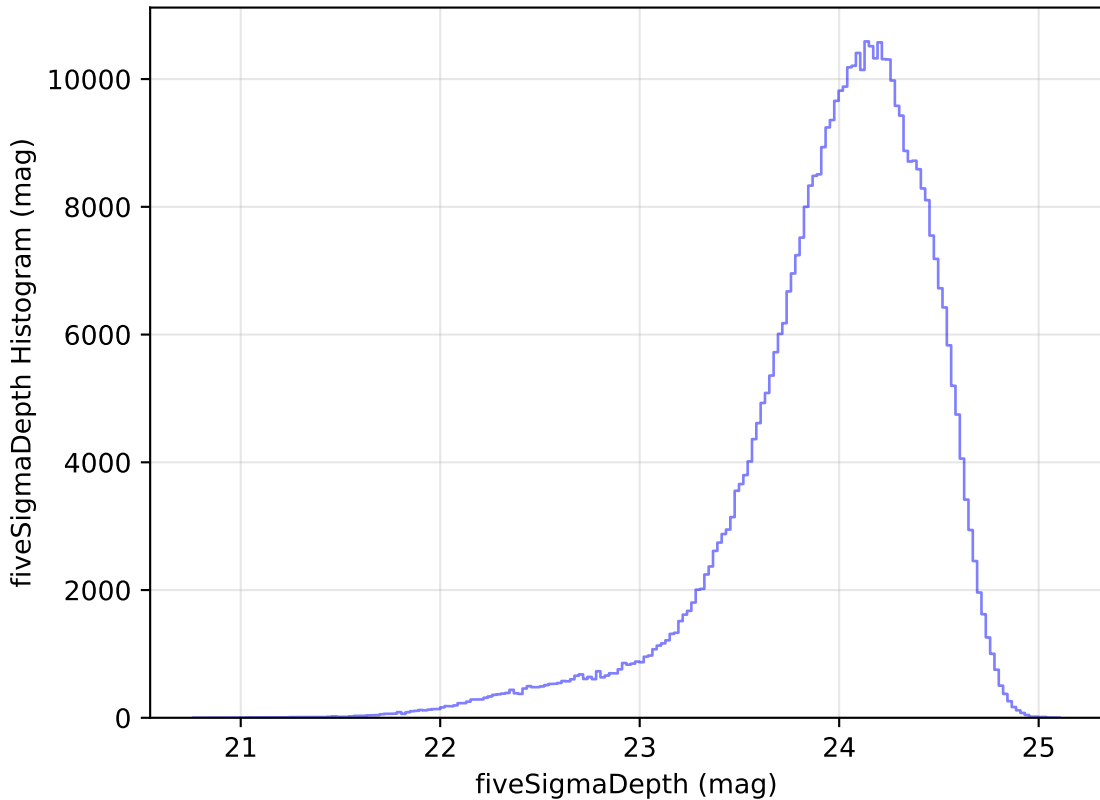
too_elab_r64_d3_griz_v3.4_10yrs All sky r band: fiveSigmaDepth Histogram
