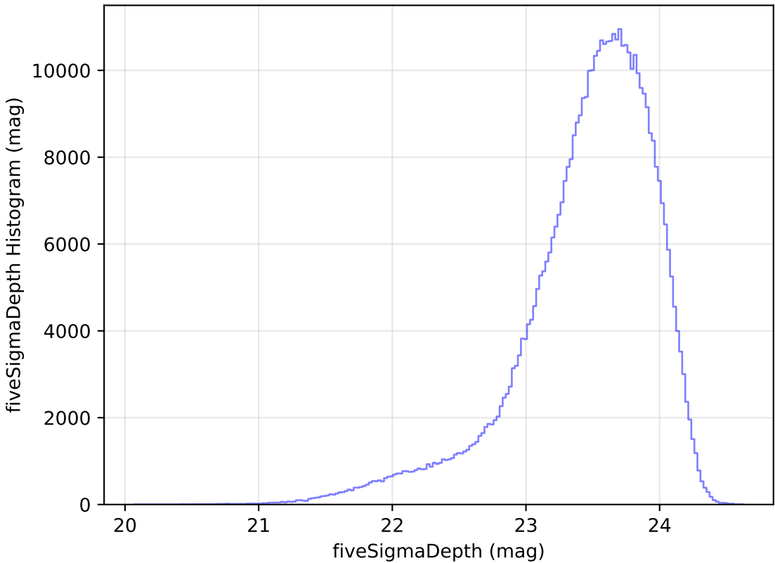
too_elab_r64_d3_griz_v3.4_10yrs All sky i band: fiveSigmaDepth Histogram
