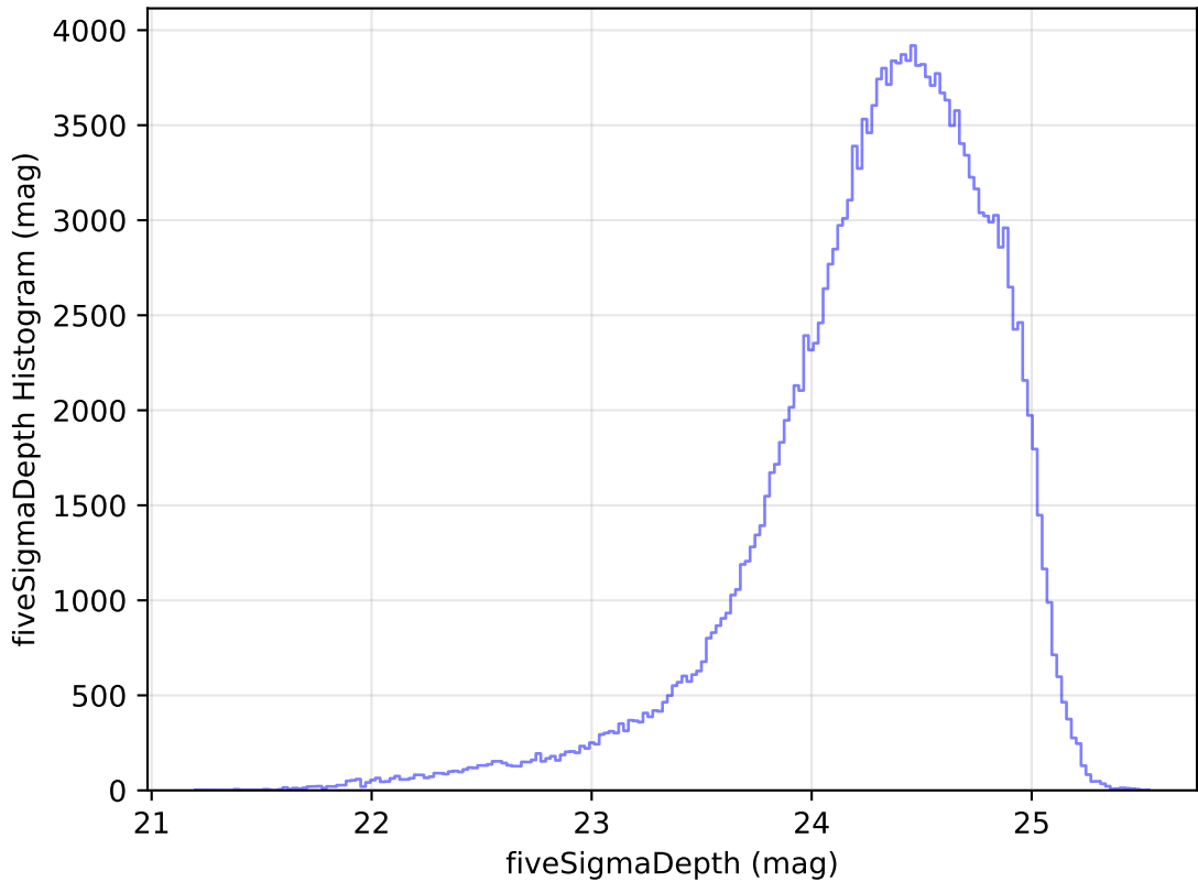
too_elab_r64_d3_griz_v3.4_10yrs All sky g band: fiveSigmaDepth Histogram
