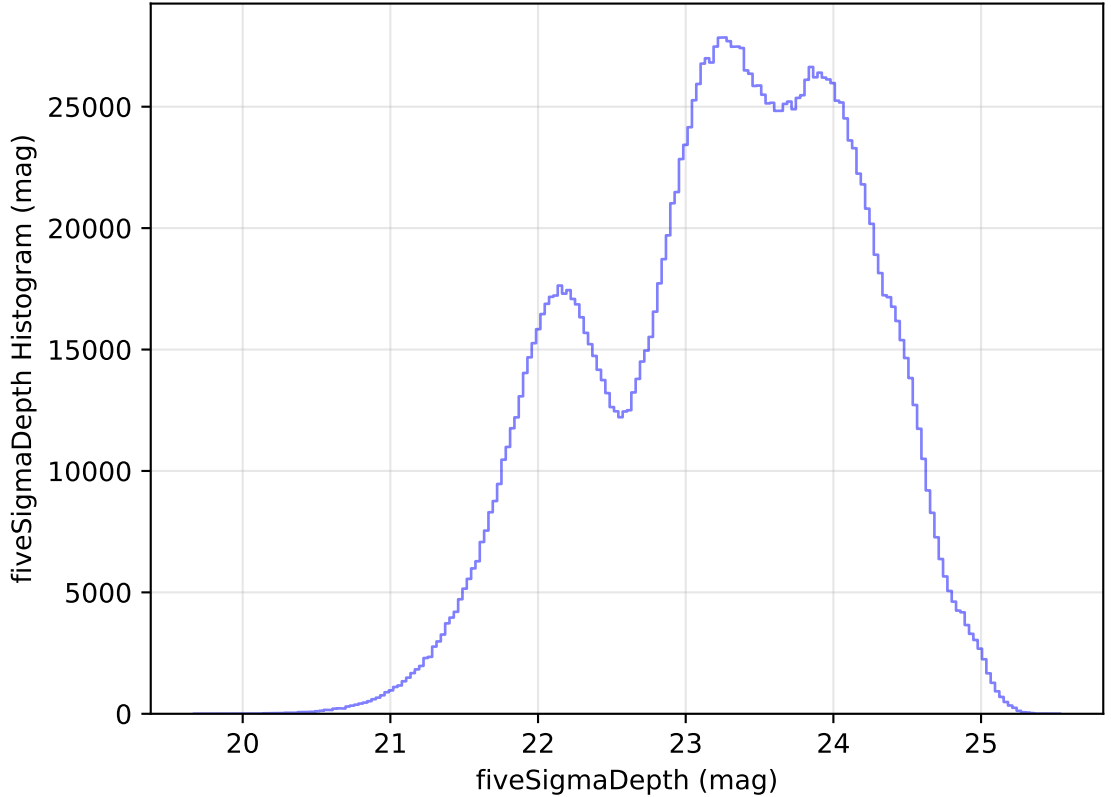
too_elab_r64_d3_griz_v3.4_10yrs All sky all bands: fiveSigmaDepth Histogram
