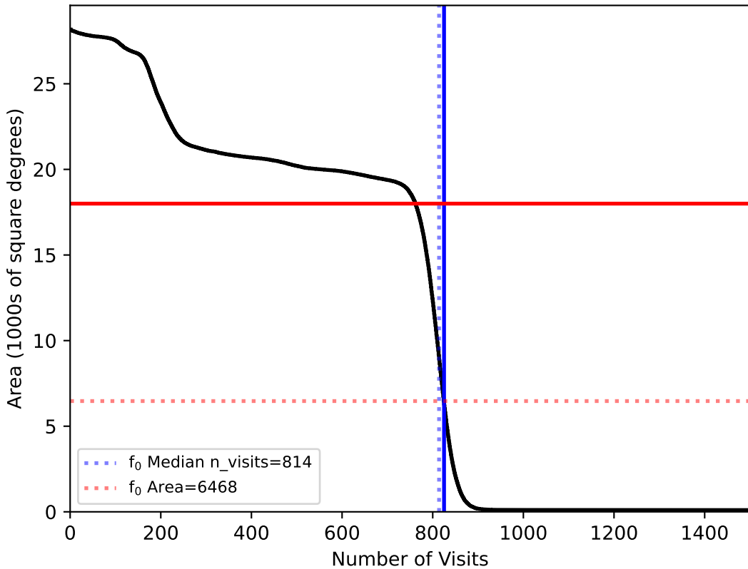
too_elab_r64_d3_griz_v3.4_10yrs All sky: fO
