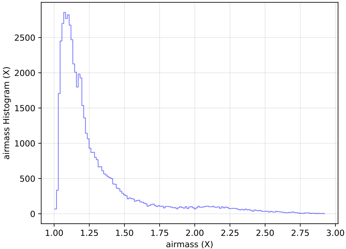
too_elab_r64_d3_griz_v3.4_10yrs Yr 1 i band: airmass Histogram
