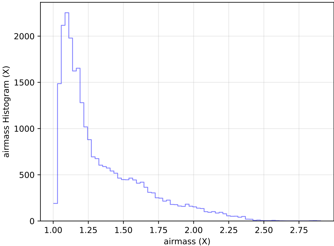
too_elab_r64_d3_griz_v3.4_10yrs Yr 1 g band: airmass Histogram
