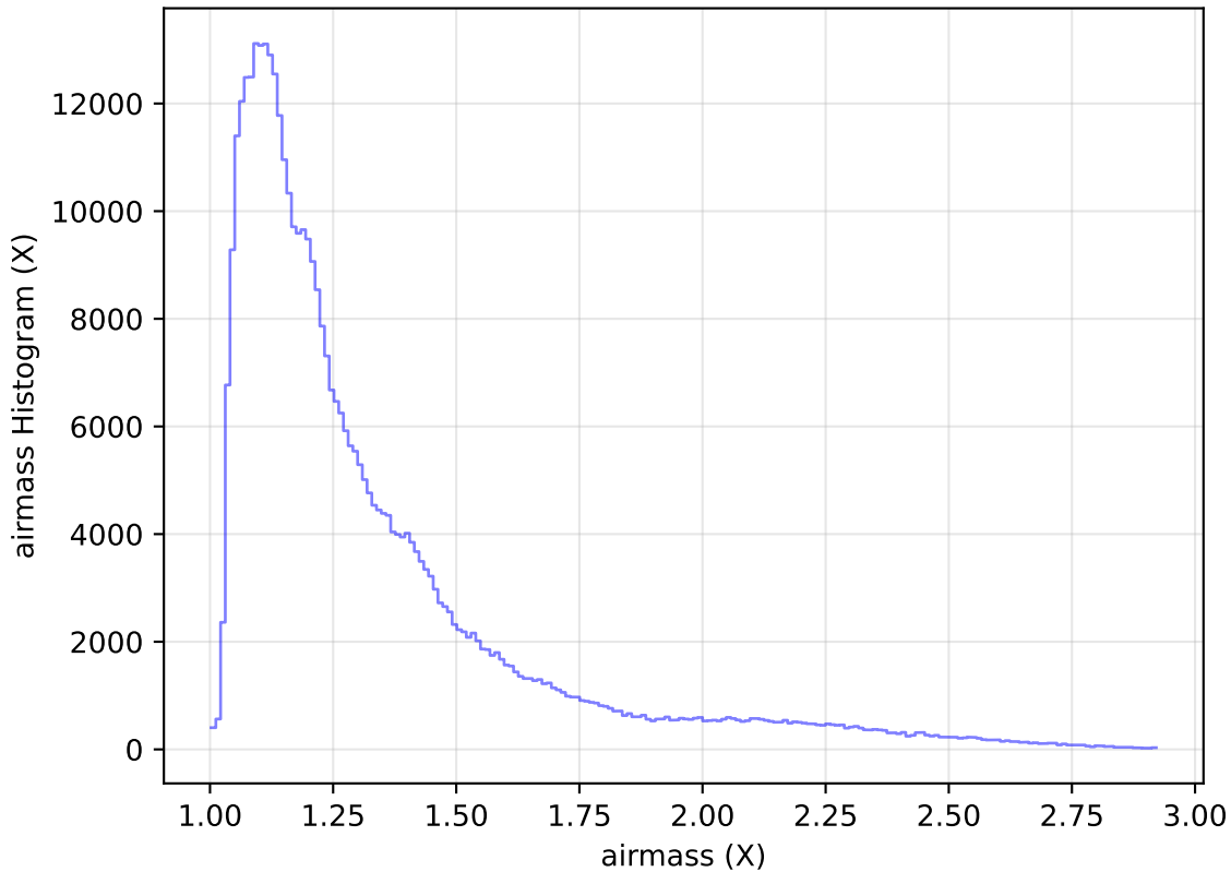
too_elab_r64_d3_griz_v3.4_10yrs WFD z band: airmass Histogram
