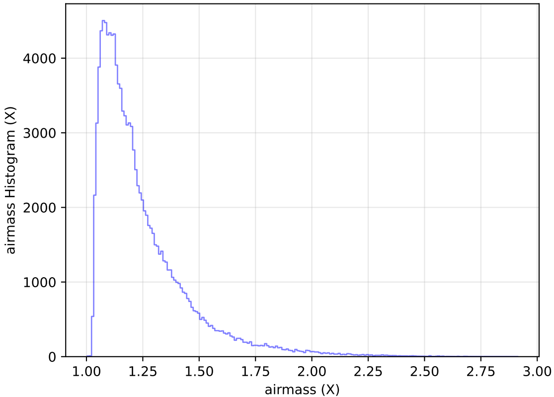
too_elab_r64_d3_griz_v3.4_10yrs WFD u band: airmass Histogram
