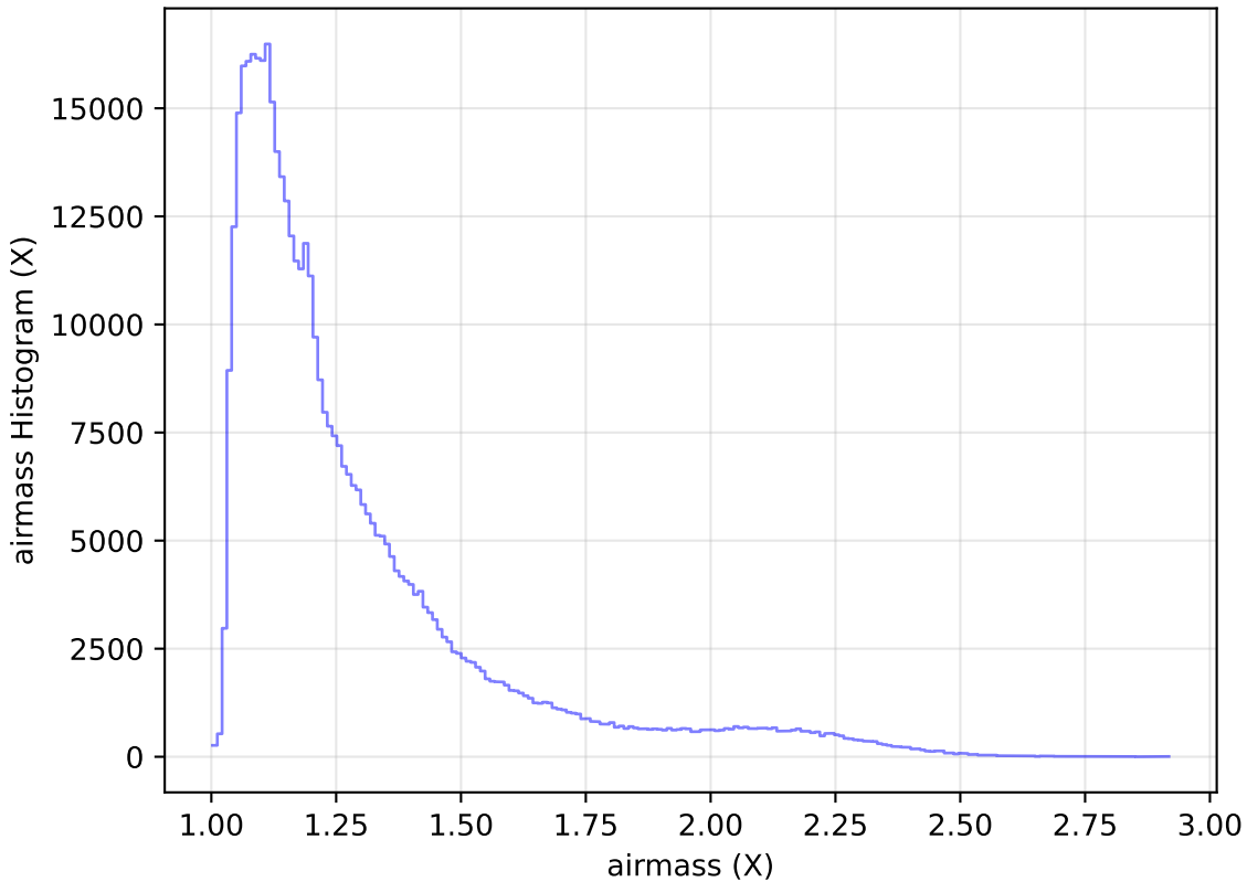
too_elab_r64_d3_griz_v3.4_10yrs WFD r band: airmass Histogram
