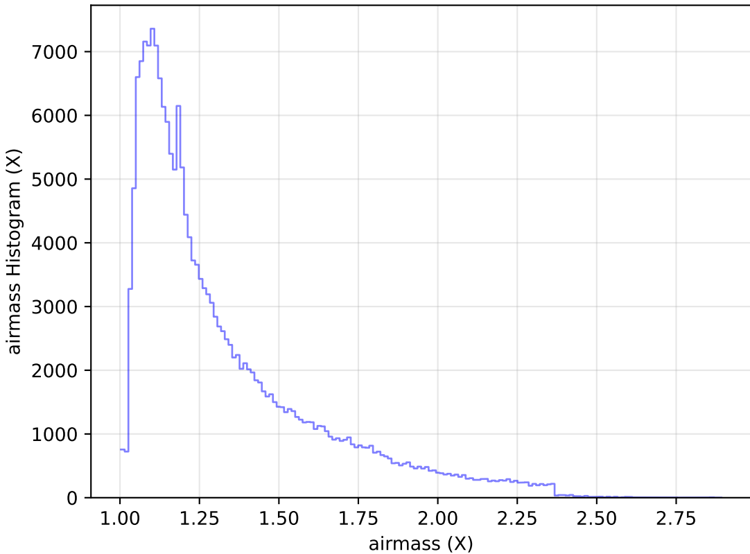
too_elab_r64_d3_griz_v3.4_10yrs WFD g band: airmass Histogram
