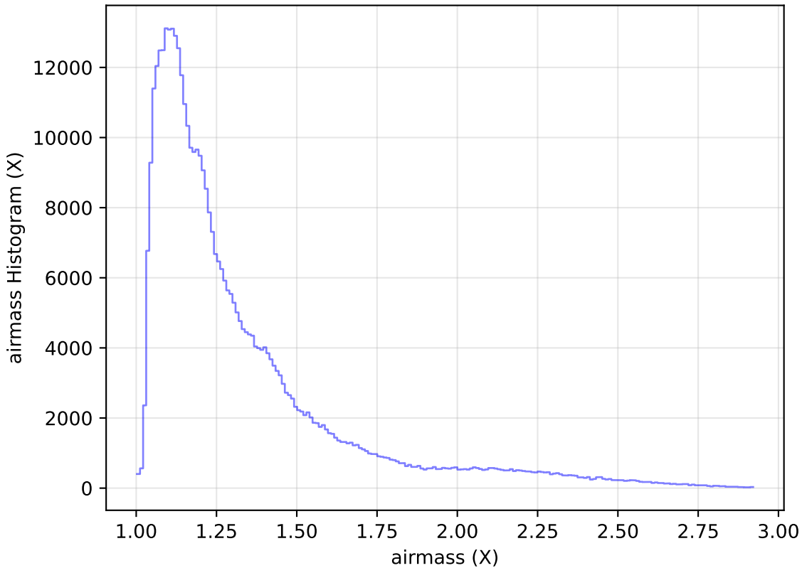
too_elab_r64_d3_griz_v3.4_10yrs All sky z band: airmass Histogram
