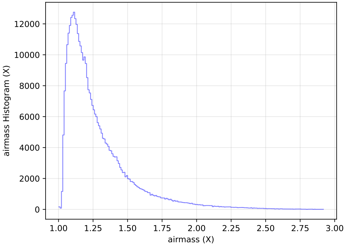
too_elab_r64_d3_griz_v3.4_10yrs All sky y band: airmass Histogram
