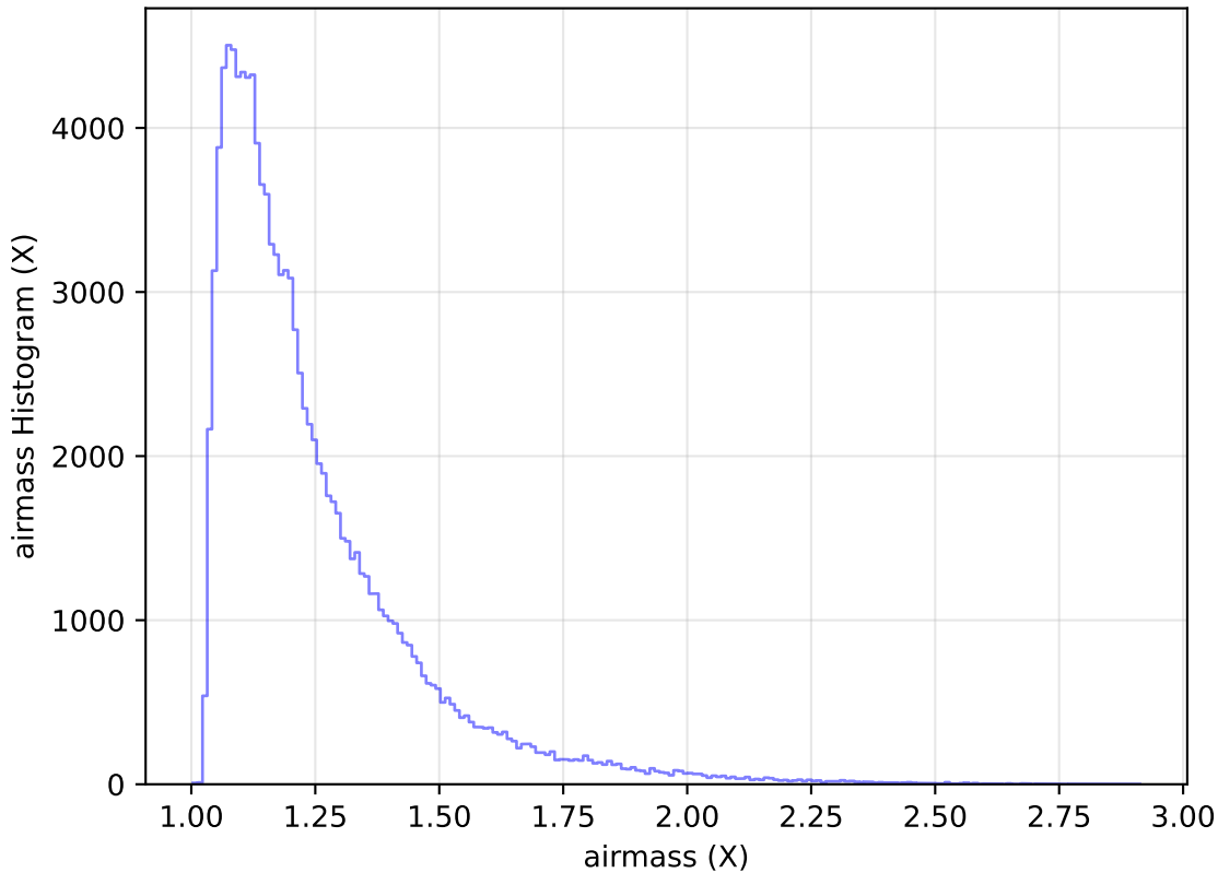
too_elab_r64_d3_griz_v3.4_10yrs All sky u band: airmass Histogram
