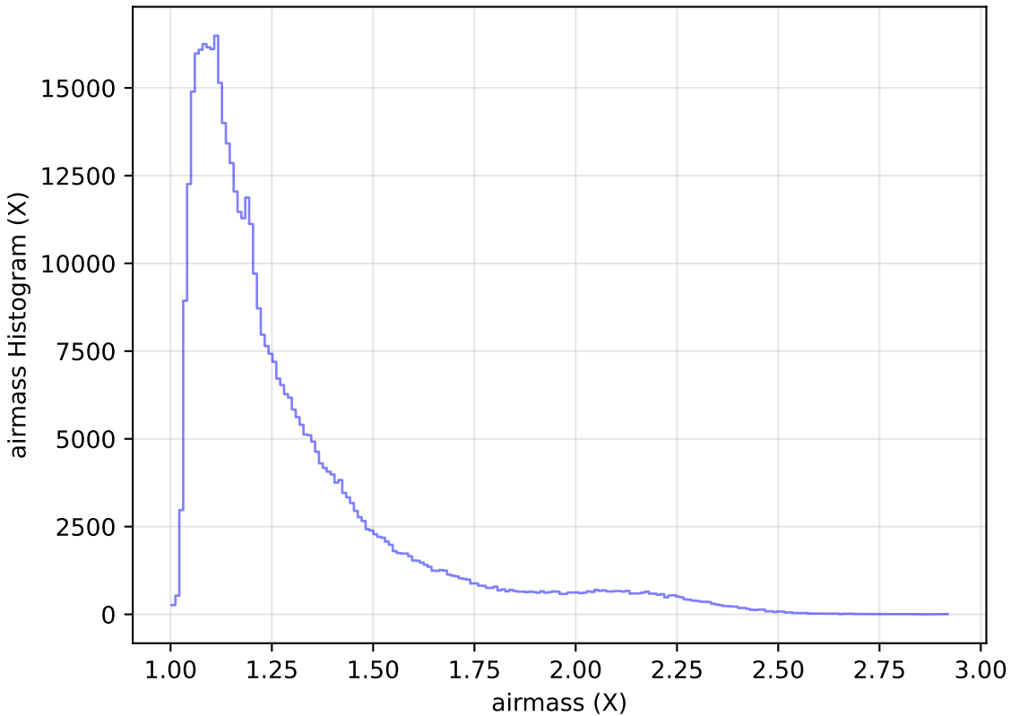
too_elab_r64_d3_griz_v3.4_10yrs All sky r band: airmass Histogram
