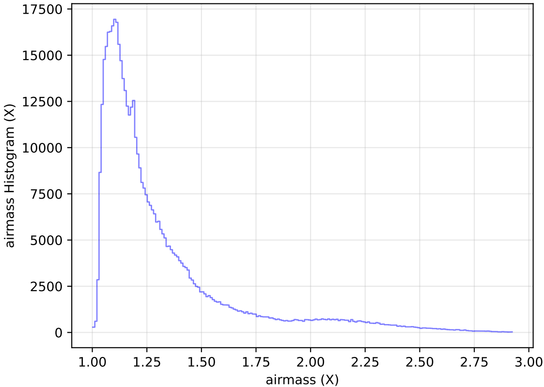
too_elab_r64_d3_griz_v3.4_10yrs All sky i band: airmass Histogram
