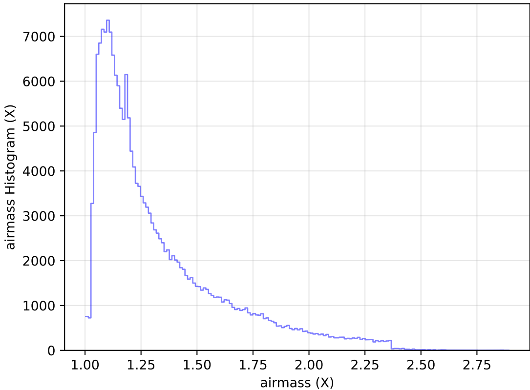
too_elab_r64_d3_griz_v3.4_10yrs All sky g band: airmass Histogram
