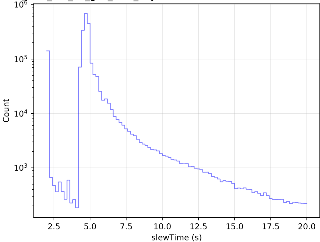
too_elab_r64_d3_griz_v3.4_10yrs All visits: Zoom Slew Time Histogram
