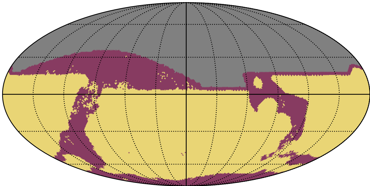
too_elab_r64_d3_griz_v3.4_10yrs All sky: RapidRevisits
