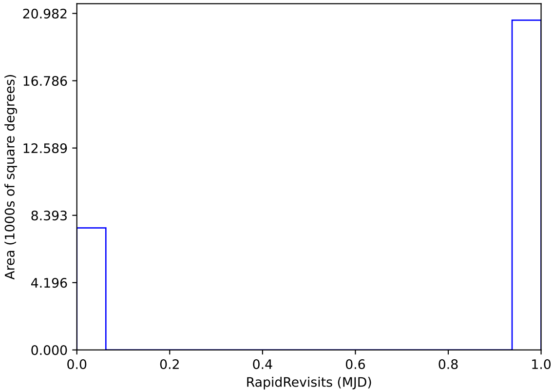
too_elab_r64_d3_griz_v3.4_10yrs All sky: RapidRevisits
