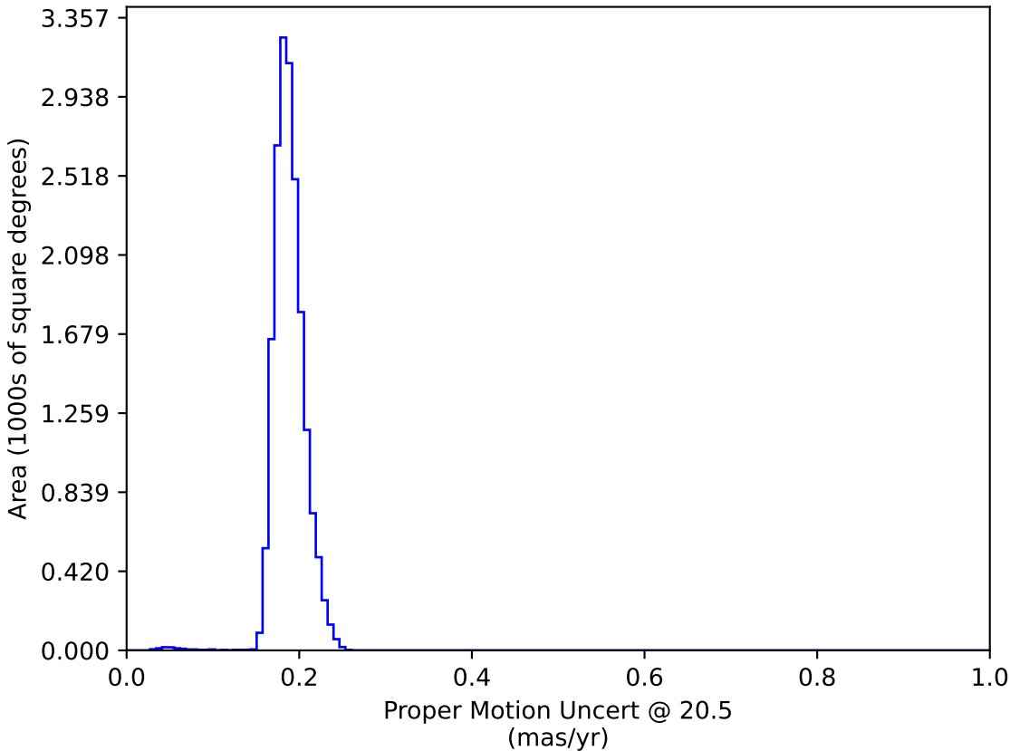
too_elab_r64_d3_griz_v3.4_10yrs WFD: Proper Motion Uncert @ 20.5
