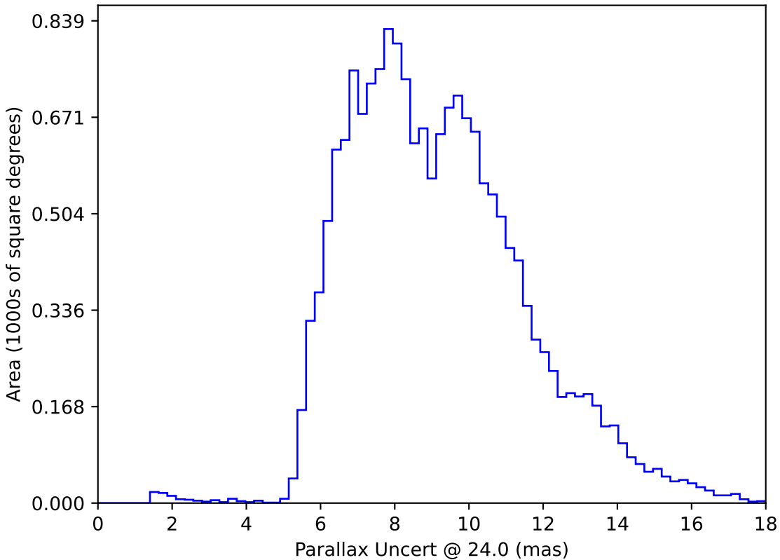
too_elab_r64_d3_griz_v3.4_10yrs WFD: Parallax Uncert @ 24.0
