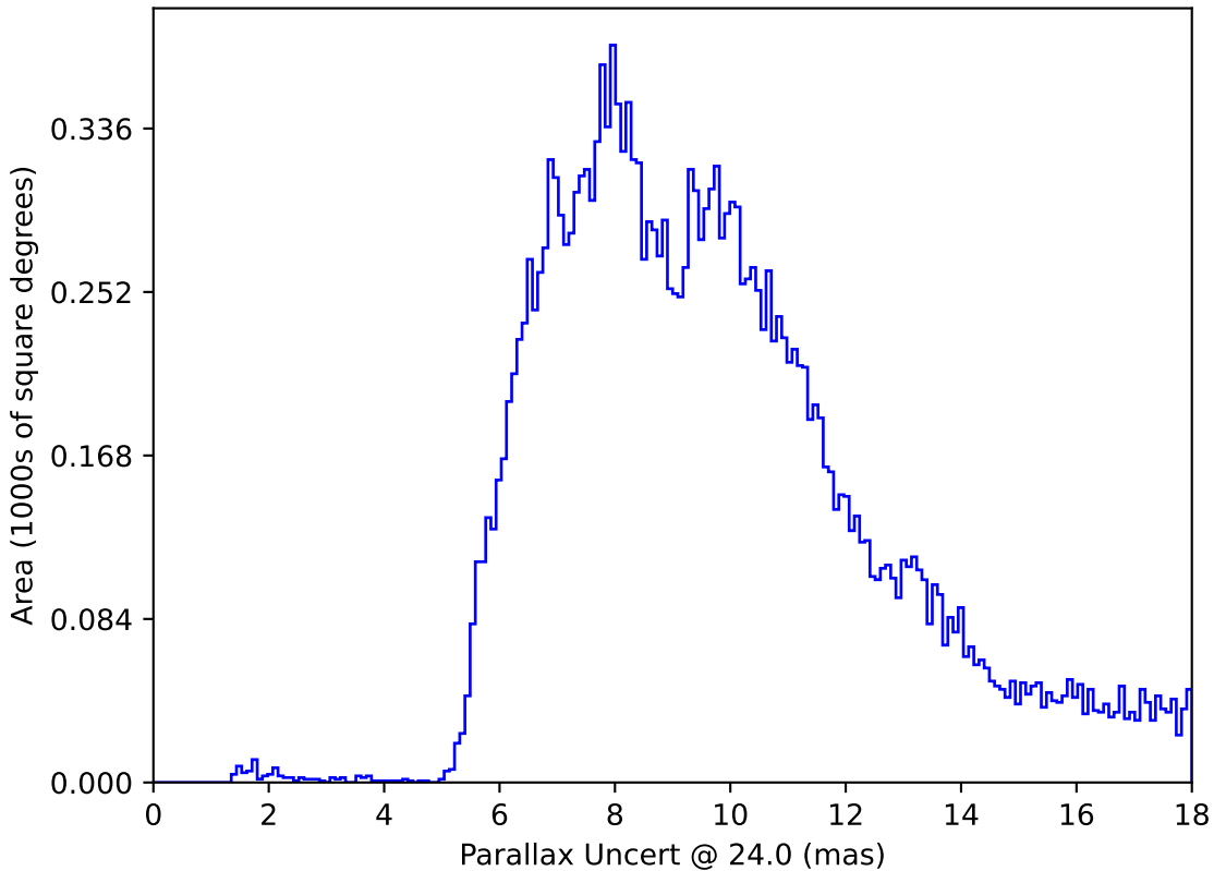
too_elab_r64_d3_griz_v3.4_10yrs All sky: Parallax Uncert @ 24.0
