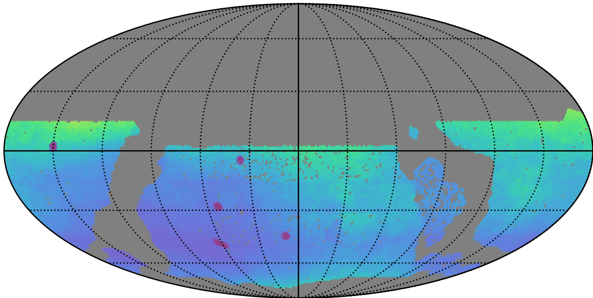
too_elab_r64_d3_griz_v3.4_10yrs WFD: Parallax Uncert @ 22.4
