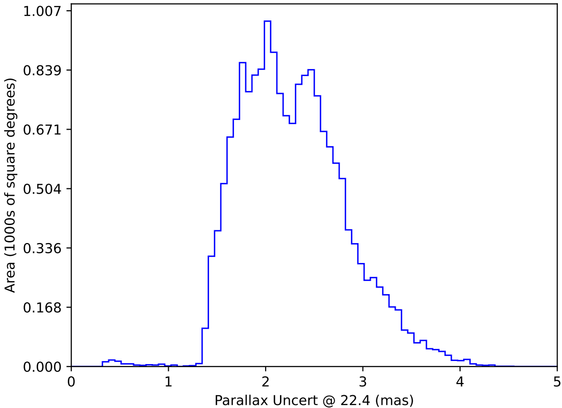
too_elab_r64_d3_griz_v3.4_10yrs WFD: Parallax Uncert @ 22.4
