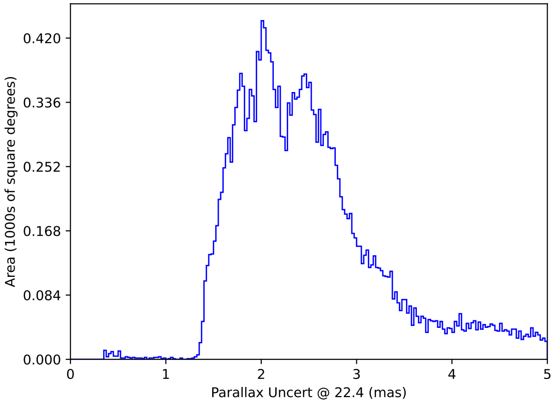
too_elab_r64_d3_griz_v3.4_10yrs All sky: Parallax Uncert @ 22.4
