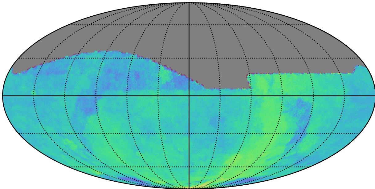
too_elab_r64_d3_griz_v3.4_10yrs All sky: Parallax Coverage @ 24.0
