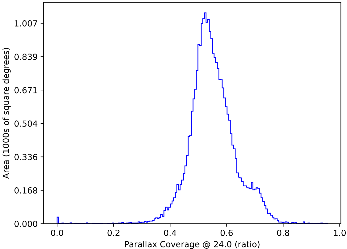
too_elab_r64_d3_griz_v3.4_10yrs All sky: Parallax Coverage @ 24.0
