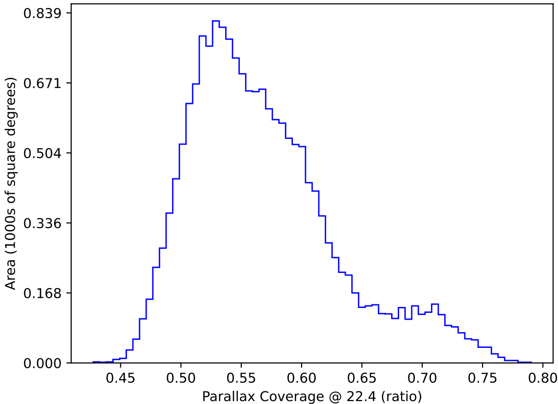
too_elab_r64_d3_griz_v3.4_10yrs WFD: Parallax Coverage @ 22.4
