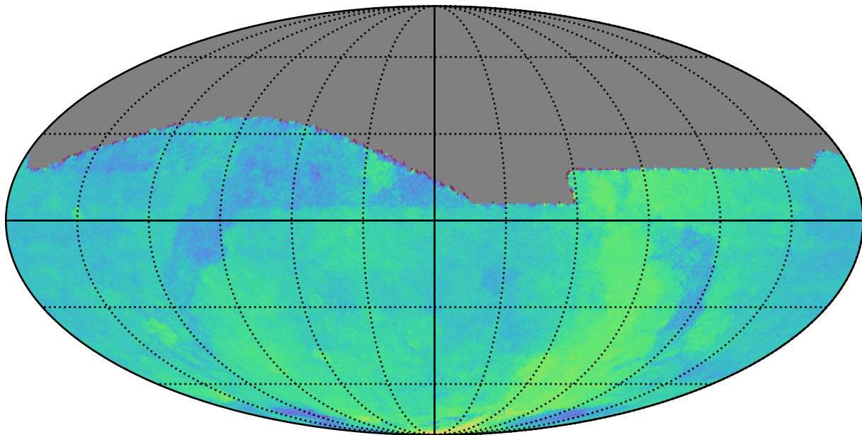
too_elab_r64_d3_griz_v3.4_10yrs All sky: Parallax Coverage @ 22.4
