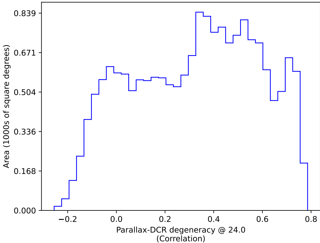
too_elab_r64_d3_griz_v3.4_10yrs WFD: Parallax-DCR degeneracy @ 24.0
