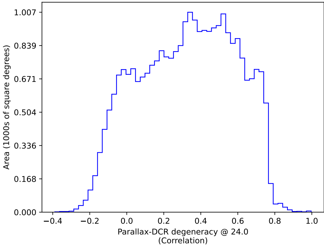
too_elab_r64_d3_griz_v3.4_10yrs All sky: Parallax-DCR degeneracy @ 24.0
