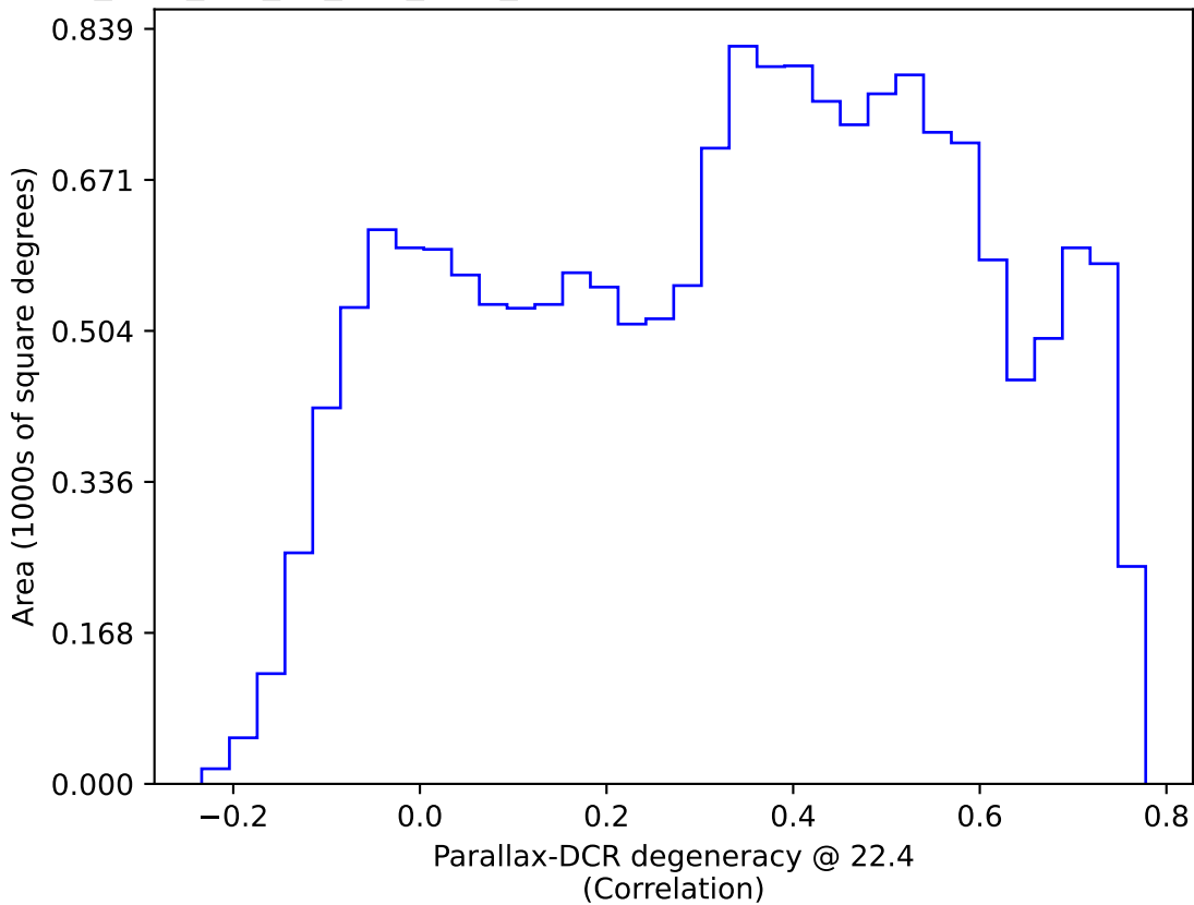
too_elab_r64_d3_griz_v3.4_10yrs WFD: Parallax-DCR degeneracy @ 22.4
