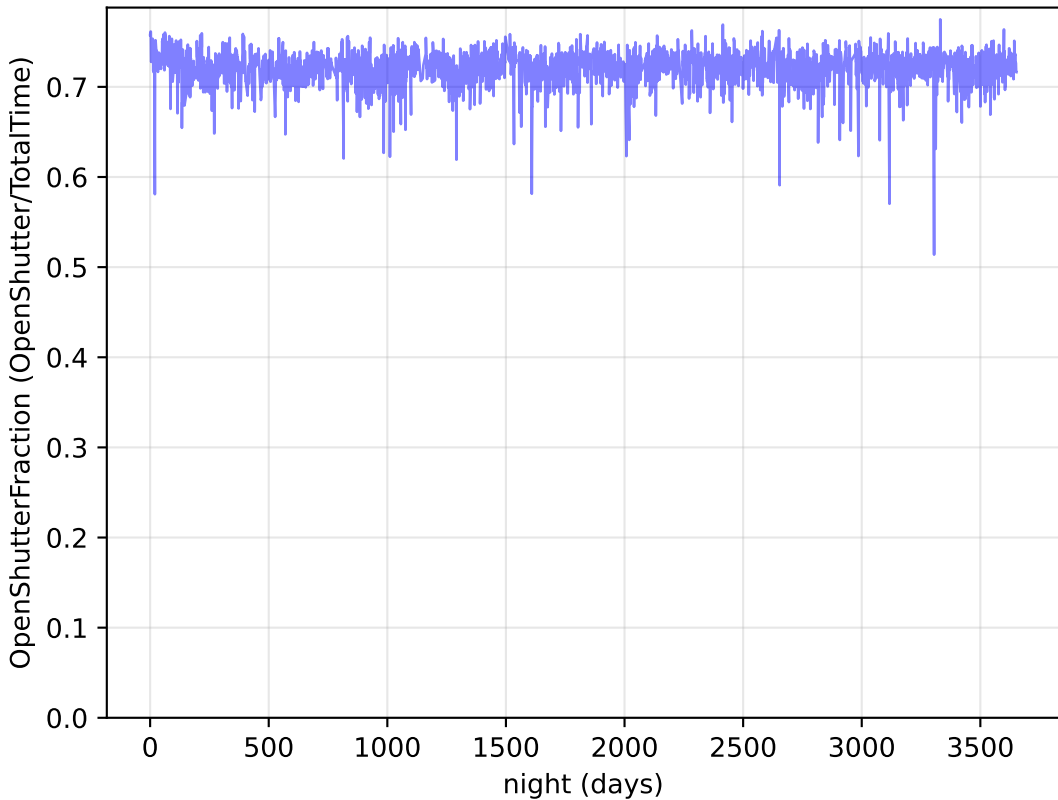
too_elab_r64_d3_griz_v3.4_10yrs Per night: OpenShutterFraction
